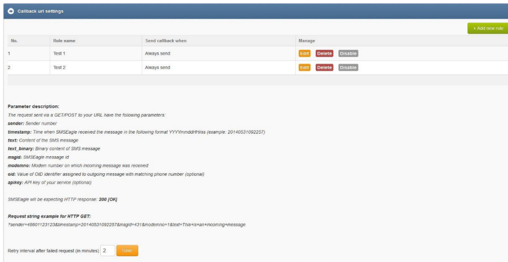
Screenshot from Callback URL settings
